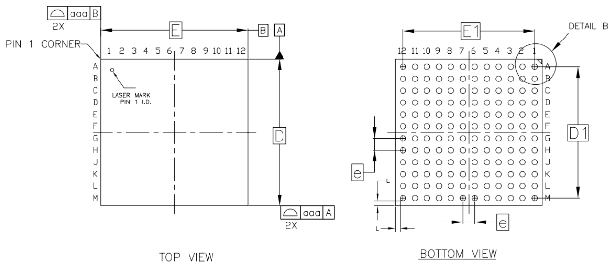
Fig. 2-2 RK628 WBBGA144 Package Top View and bottom View
