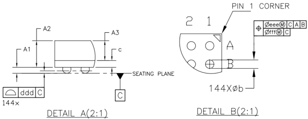
Fig. 2-4 RK628 WBBGA144 Package side View
