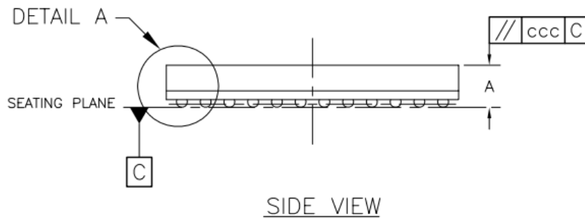
Fig. 2-3 RK628 WBBGA144 Package side View
