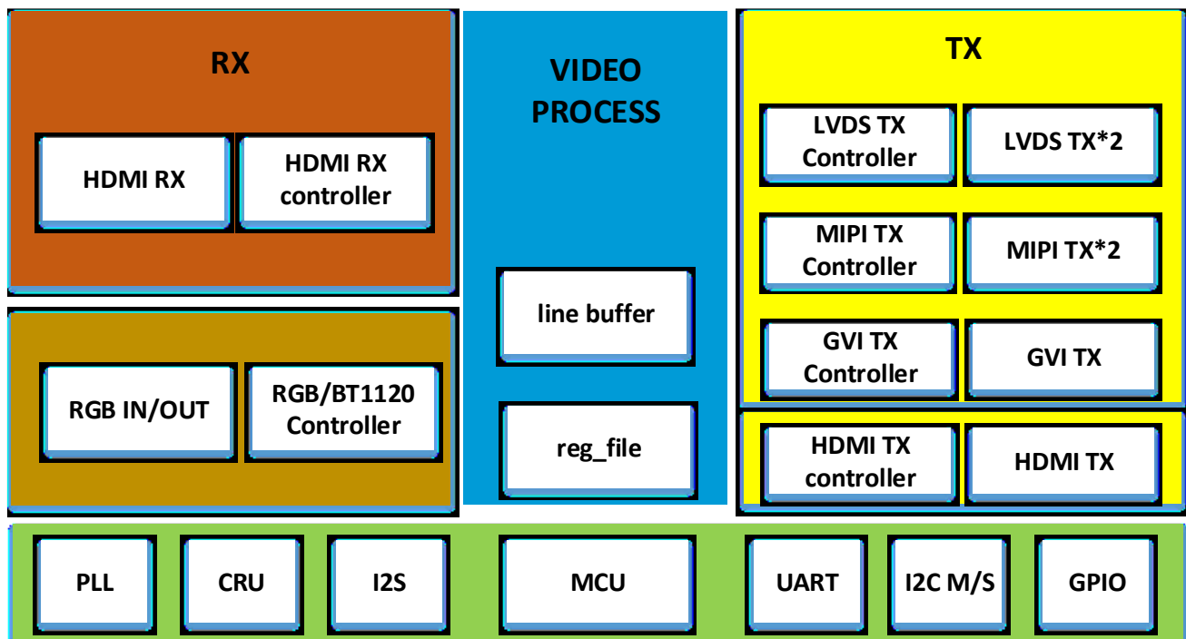
Fig. 1-1 RK628 Block Diagram
