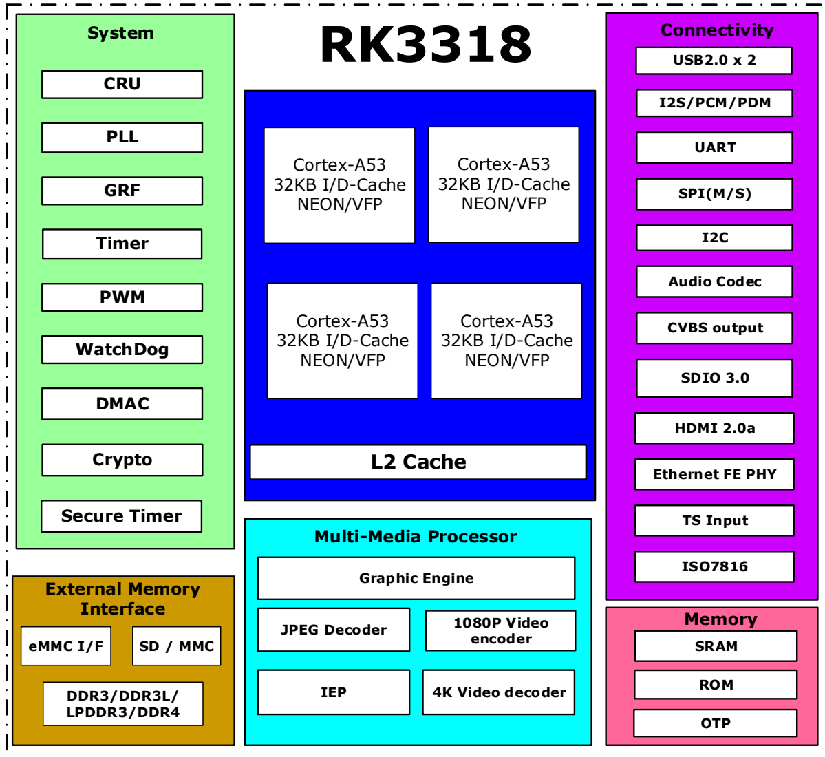
Fig.1-1 Block Diagram
