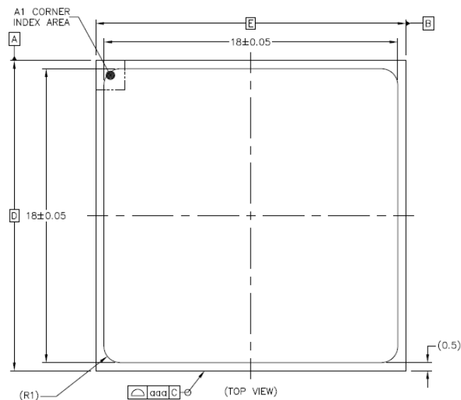
Fig. 2-12 RK3288 FCCSP636LD Package Top View--EOL
