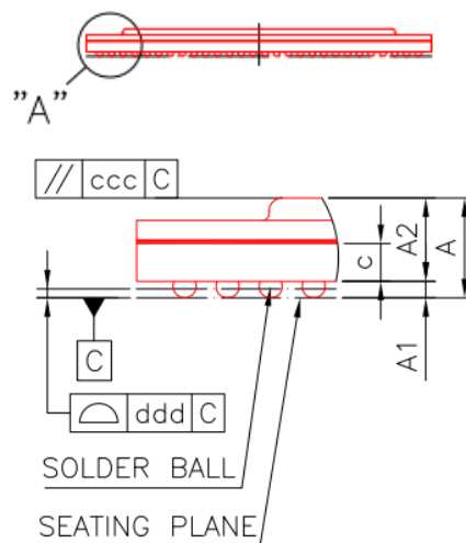
Fig. 2-10 FCBGA636LD Package Side View
