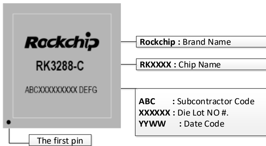
Fig. 2-3 RK3288-C Silk Marking
