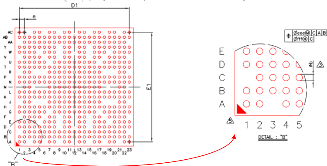
Fig. 4 RK3066/RK3066A TFBGA453 Package Bottom View
