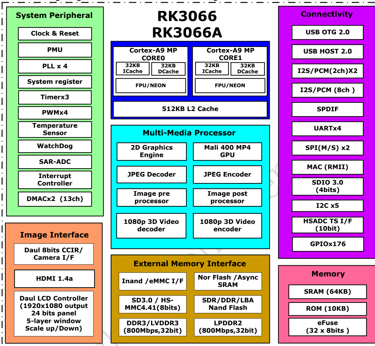
Fig. 1 RK3066/RK3066A Block Diagram
