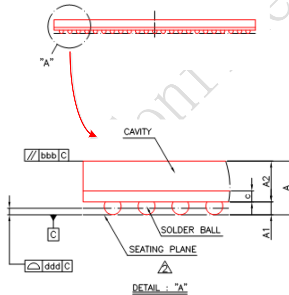
Fig. 2 RK3066/RK3066A TFBGA453 Package Side View
