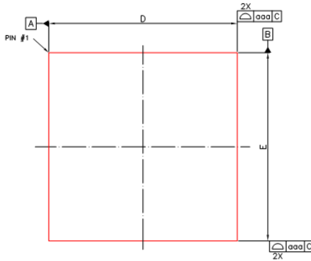
Fig. 2 RK3066/RK3066A TFBGA453 Package Top View
