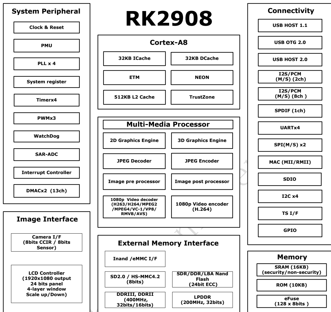
Fig. 1-1 RK2908 Block Diagram
