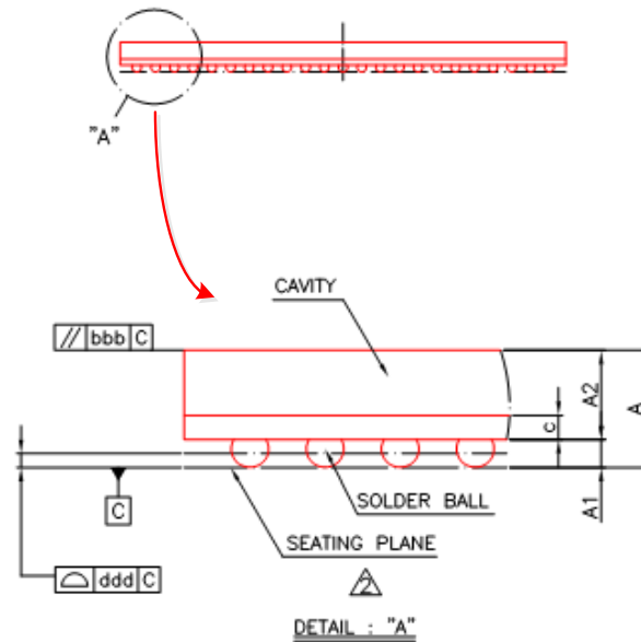
Fig. 2-2 PX3 TFBGA453 Package Side View
