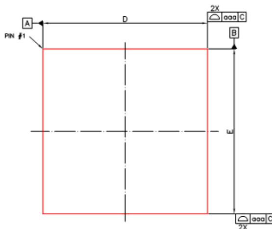
Fig. 2-1 PX3 TFBGA453 Package Top View
