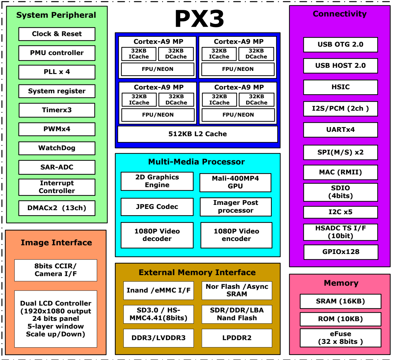
Fig. 1-1 PX3 Block Diagram
