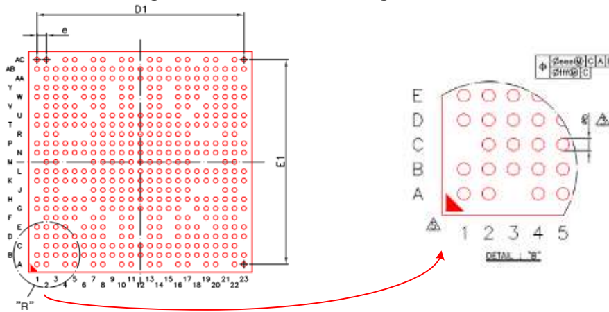
Fig. 2-3 PX3 TFBGA453 Package Bottom View
