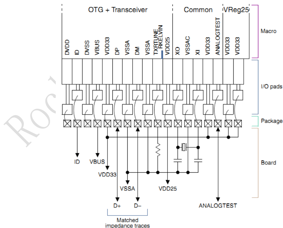
Fig. 4-3 RK PX2 USB OTG/Host2.0 interface reference connection
